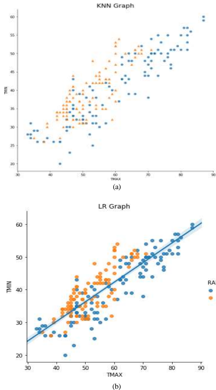
Figure 5. Comparing scatter graph results for weather prediction in (a) k-nearest neighbor and (b) logistic regression
